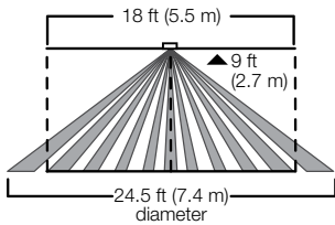
Vertical view
