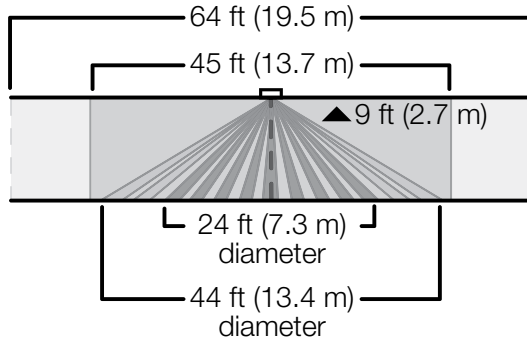
Vertical view
